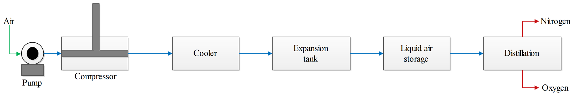
Figure: Manufacture of Nitrogen and oxygen by Linde's process
